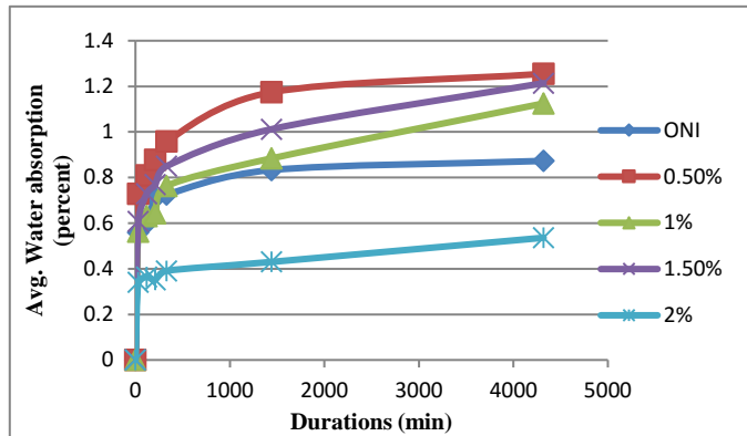
Fig 7 Water absorption in OC
