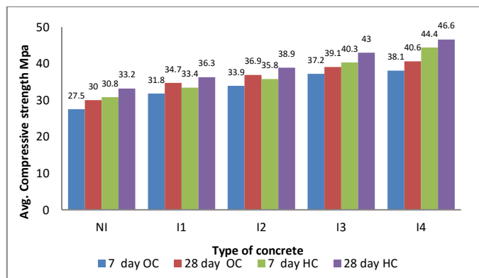
Fig 4(b) Compressive Strength of concrete cylinders
