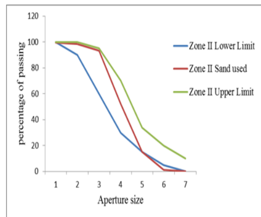
Fig 2. Zone II grade of sand
