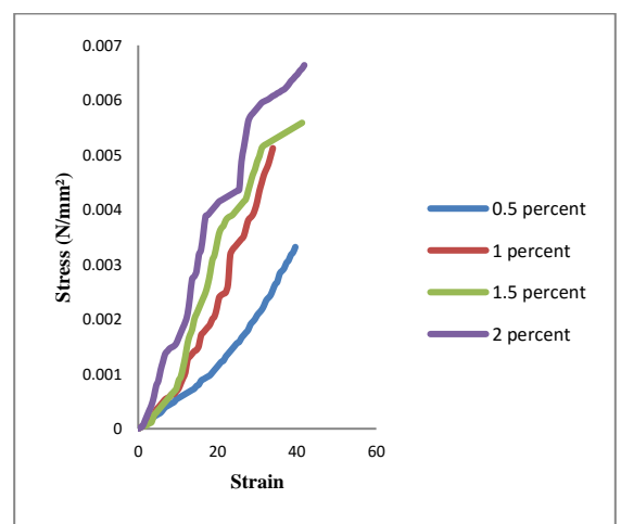
Fig 6 Graphs for Modulus of Elasticity for OC
