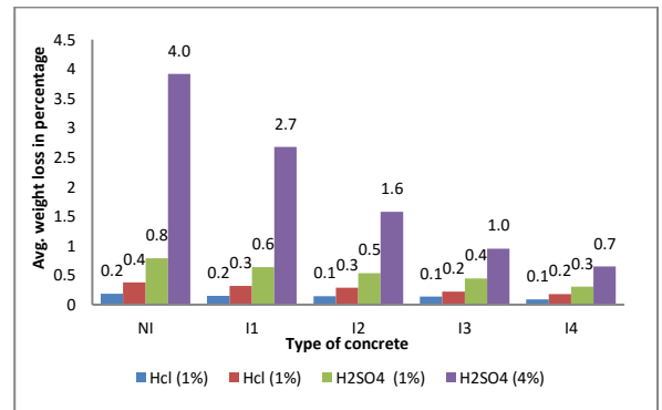
Fig 10 Acid Resistance result for HPC
