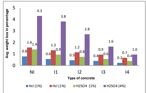
Fig 9 Acid Resistance result for OC
