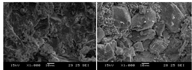
(a).OC without inhibitor Fig (b). HPC without inhibitor
