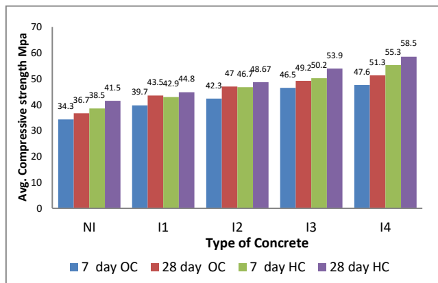
Fig (a) Compressive Strength of concrete cubes
