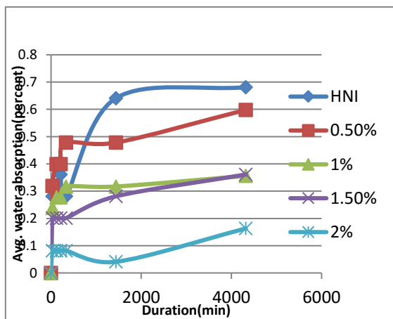
Fig 8 Water absorption in HPC
