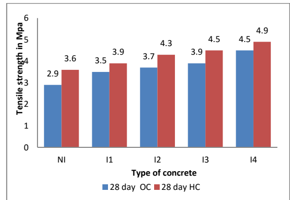
Fig 5 Split Tensile Strength of concrete cylinders
