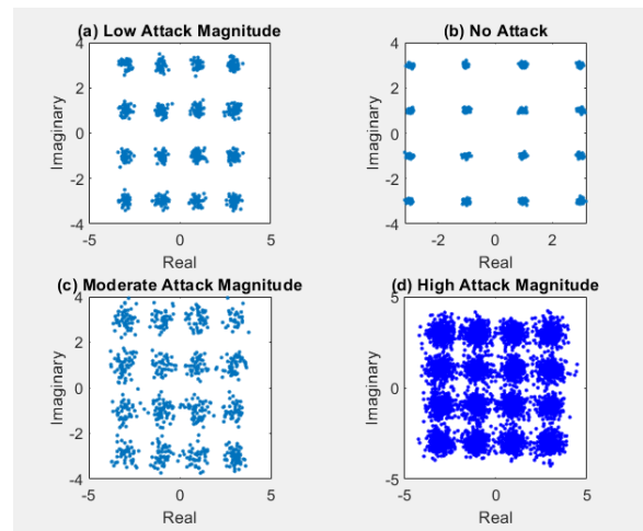
Fig.5 Scatter Plots
