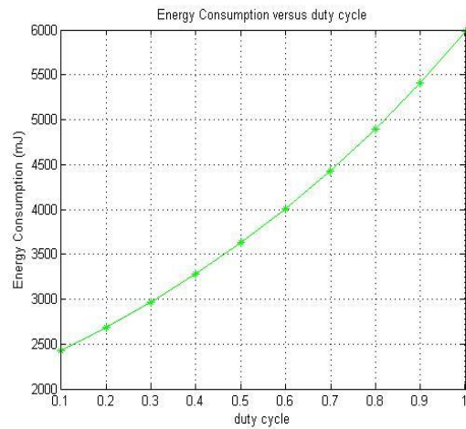
Fig.6 Energy Consumption versus duty cycle for r=100
