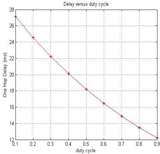
Fig.4 One hop Delay versus duty cycle
