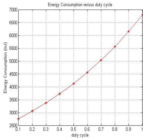
Fig.7 Energy Consumption versus duty cycle for r=120
