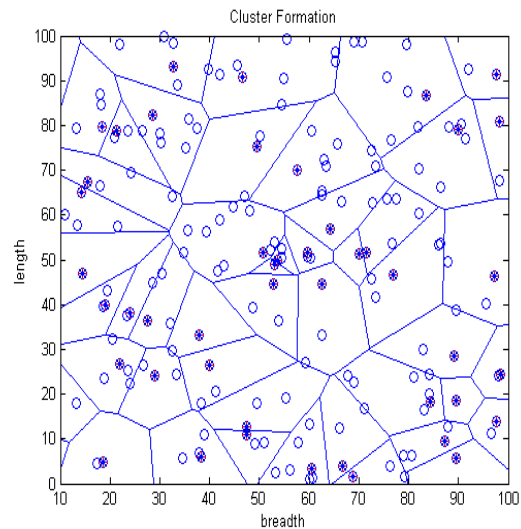
Fig.2 Initial Clustering
