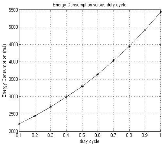
Fig.5 Energy Consumption versus duty cycle for r=80
