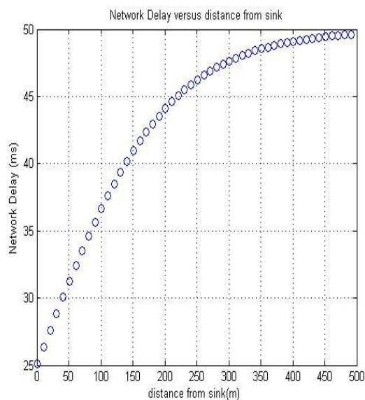
Fig.9 Network Delay versus distance from sink
