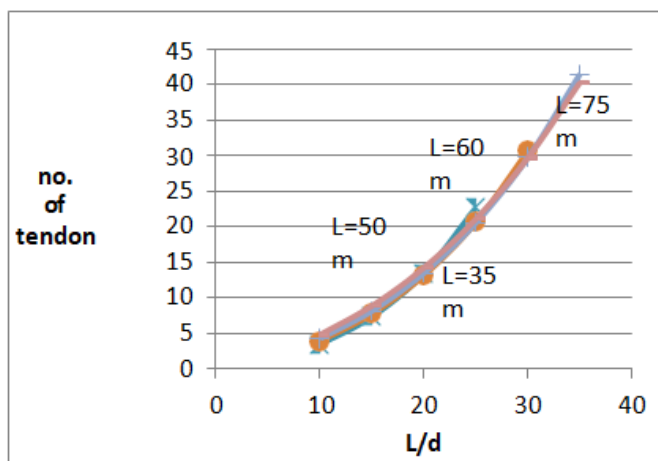
Graph4.3Variationofno.ofstrandwithspan by depth ratio
