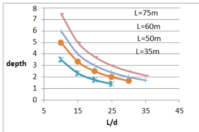
Graph4.2Variationofspan to depth ratio for different span with depth
