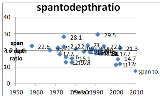
Graph3-1variationofspantodepthratioof box
