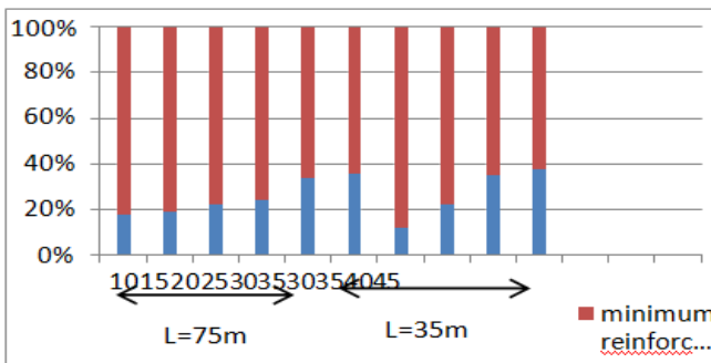
Graph 5.8 Cost distribution of reinforcement and stirrups
