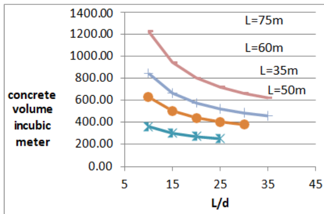
Graph4.1Variationofconcretevolumewithspan by depth ratio for different span
