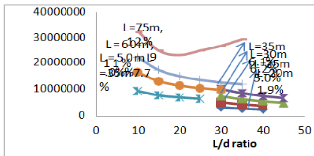
Graph 5.10 Total construction cost comparison
