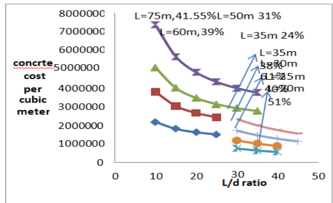
Graph 5.5 Comparison of Cost of Concrete
