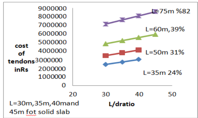
Graph 5.4 variation of cost of tendons
