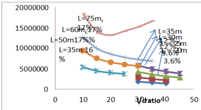
Graph 5.9 Total concrete of superstructure cost comparison
