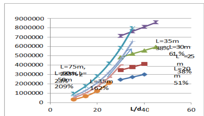
Graph 5.6 Comparison of Prestressing Tendon Cost
