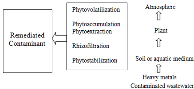
Fig.1. The uptake mechanism of phytoremediation
