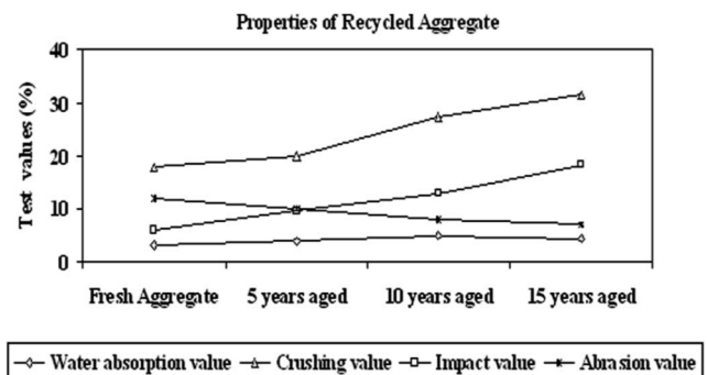
(Figure 1: Comparison of Natural aggregate and Recycled aggregate Mechanical Properties, P.Saravana kumar et al. (2012)).
