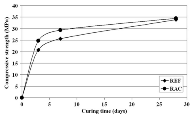
(Figure 5: Comparison of NCA and RCA with compressive strength) (Behaviour of beam column joints made of recycled aggregate concrete under cyclic loading (valeria corinaldesi et al. 2010))
