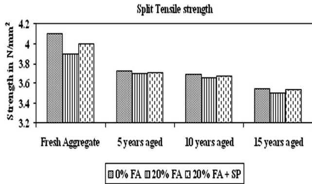
(Figure 6: Effect of admixed recycled aggregate concrete on properties of fresh and hardened concrete by P.Saravanakumar and G. Dhinakara.)
