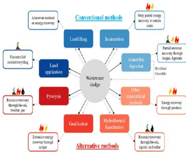
Figure 3. Alternative ways of waste to energy conversion [9]
