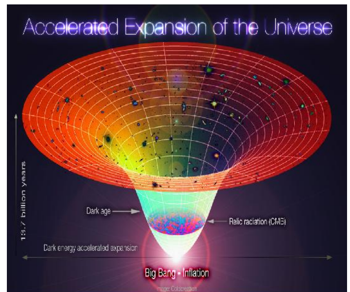
Figure 4: Diagram showing the Lambda-CDM universe from the Big Bang to the current era
