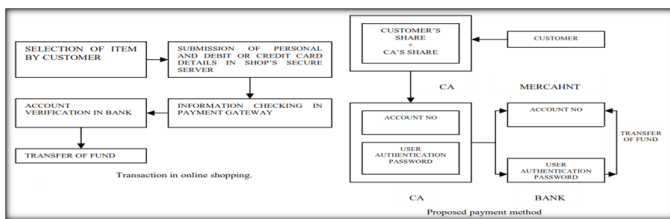
Fig:2.system architecture
