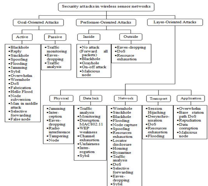
Fig.1. Security attacks in wireless sensor networks
