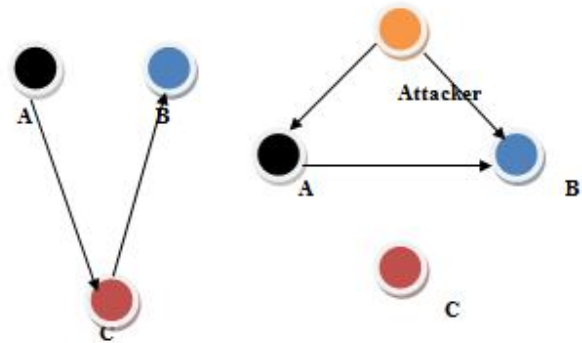
Fig 4 Wormhole Attack
