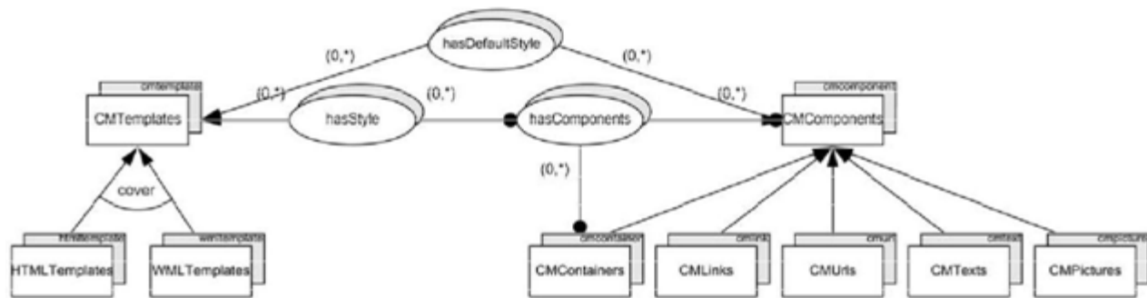
Figure 3: Association of Document Components and Templates
