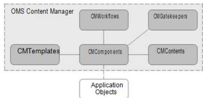
Figure 2: OMS Java CMS Schema Parts
