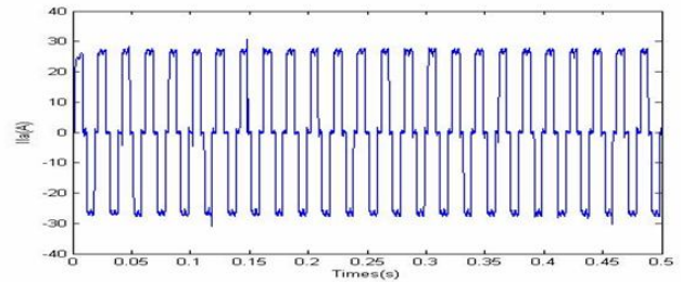
Figure 6 line current
