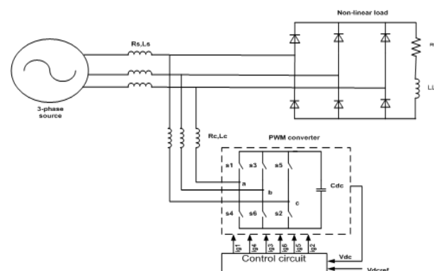
Figure 3. Schematic diagram of shunt active filter.
