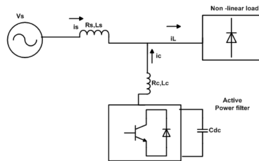
Fig 1. Shunt active power filters Basic compensation principle
