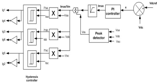
Figure 4. APF Control Scheme with PI Controller
